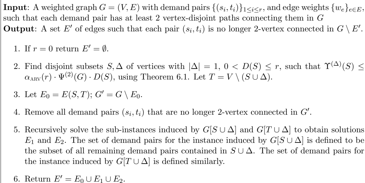
Figure 6: Approximation algorithm for VC-kRC, k = 2 (weighted case).
