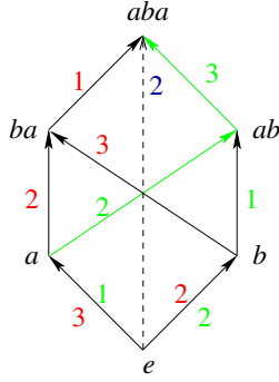
Figure 2: [e, aba] is BW-labelable. The path (e < aba) has label \lambda_1((e < aba)) = 2 .
