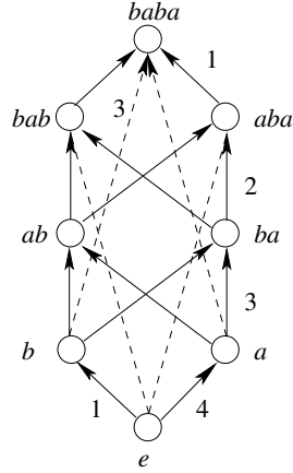
Figure 3: B(u, v) with u = e , v = baba = abab with u, v \in I_2(4) .
