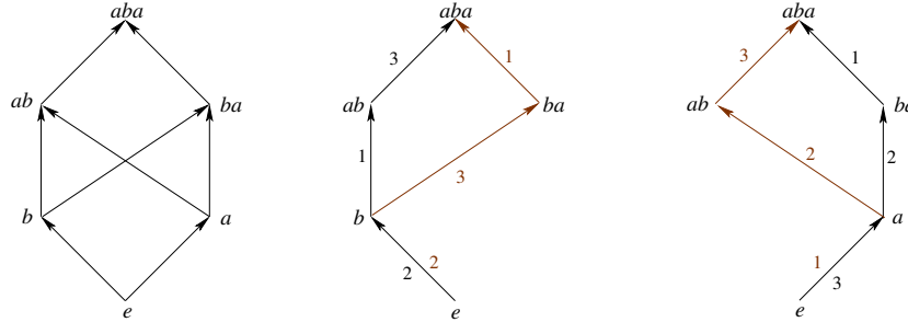
Figure 1: Björner and Wachs's labeling for maximal-length paths of B(e, aba) . Notice that the edge (e < a) has two possible labels depending on which "a" is removed from aba .
