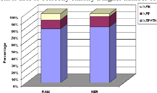
Fig. 2. Percentage of correct classifications, false positive and false negative errors.
