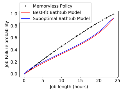
Fig. 9: Impact of suboptimal bathtub model parameters on the scheduling policy is negligible.
